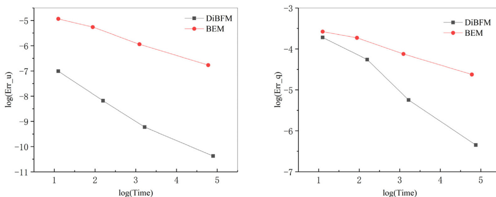
Fig. 10. Comparison of efficiency between DiBFM and Tradition BEM.
