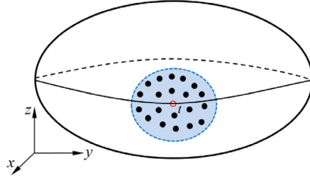
Fig. 5. Point t and its neighborhood.
