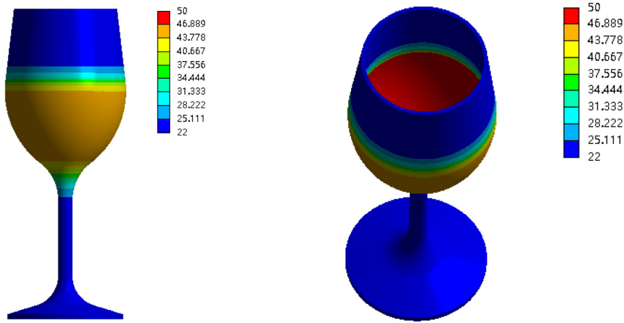
Fig. 13. Contours of temperature: FEM with 222335 nodes.
