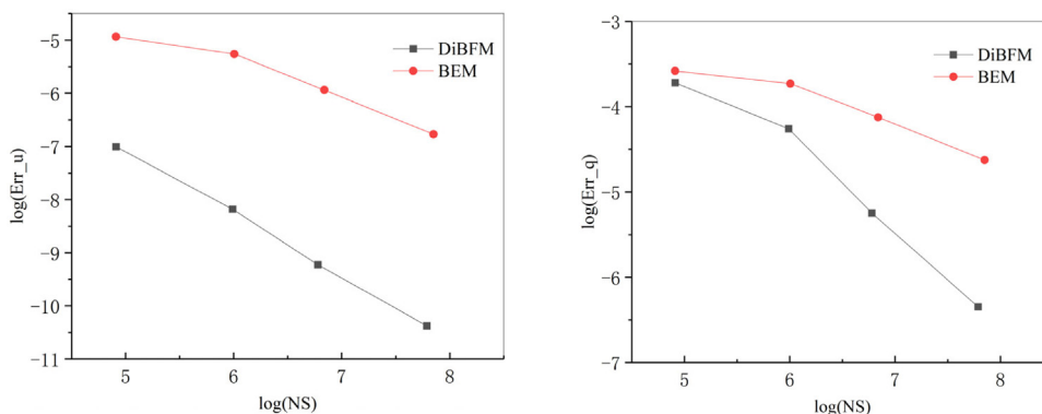
Fig. 9. Comparison of accuracy between DiBFM and Tradition BEM.
