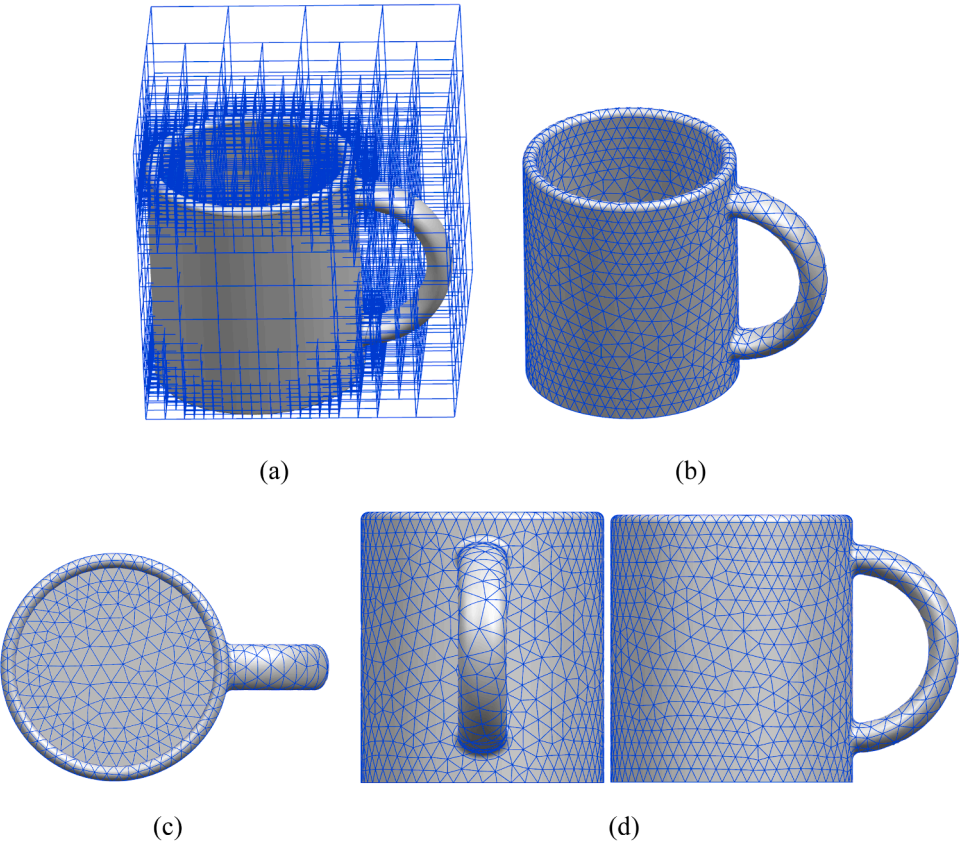
Fig. 39. Results of the cup meshed by AFM: (a) Sizing field constructed by octree refinement; (b) Front view; (c) Top view; (d) Side view.
