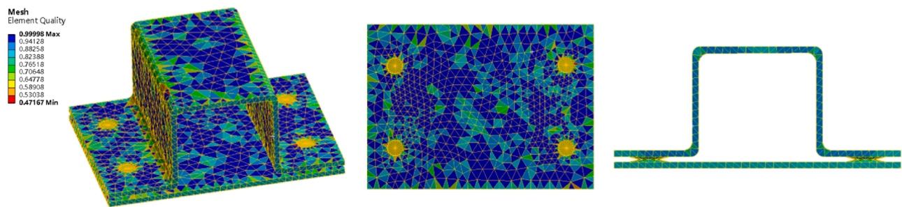
Fig. 45. Results of the spot-welding model meshed by ANSYS workbench.
