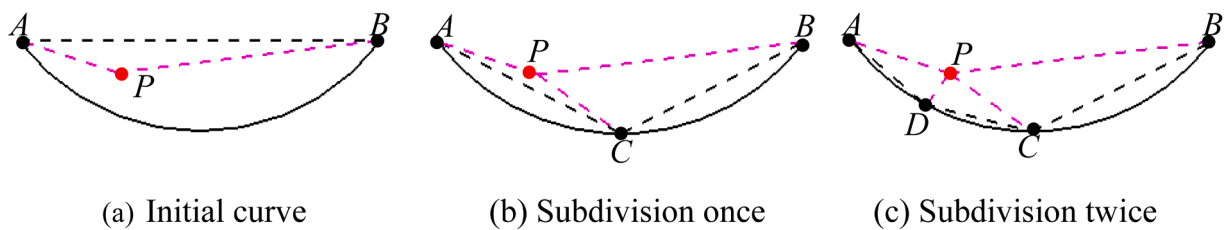
Fig. 17. Subdivision process of curve while a point lies in the area between a curve and its chord.
