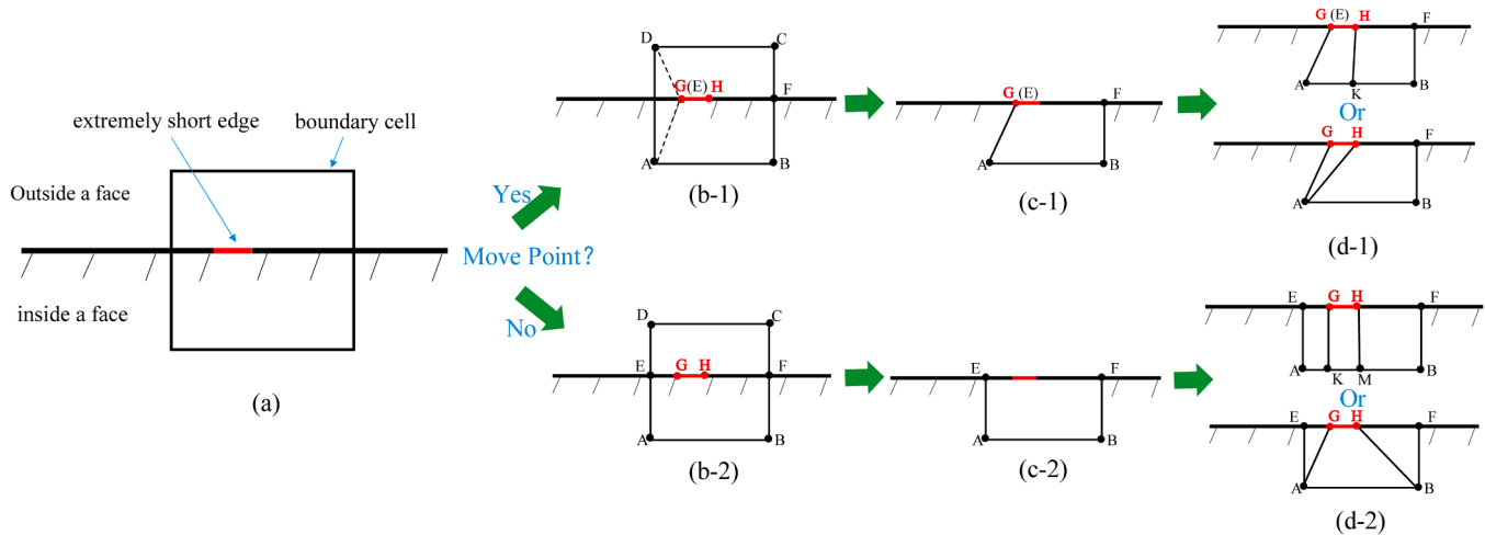
Fig. 48. BTM process for extremely short edges.
