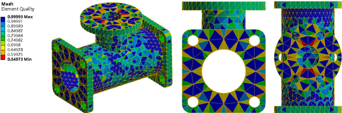
Fig. 36. Results of three-way pipe meshed by ANSYS workbench.
