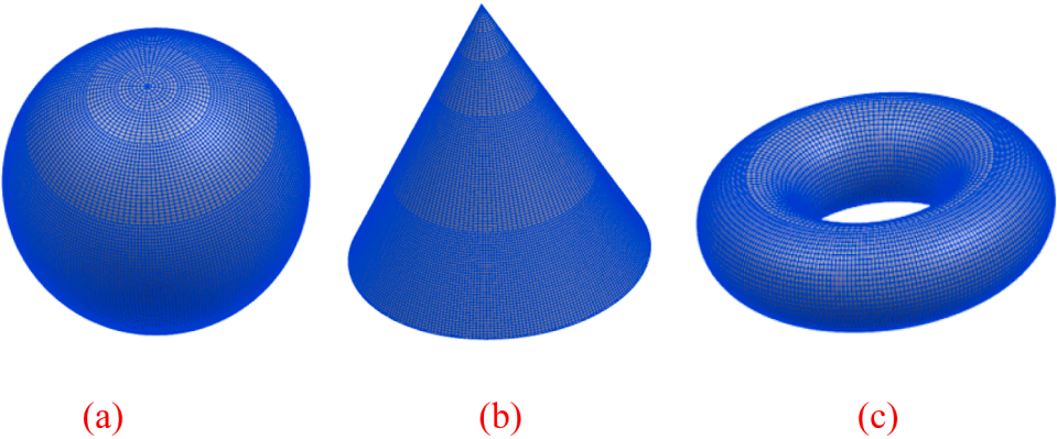
Fig. 30. Mesh results of BTM:(a) Sphere (mesh number:19936); (b) Cone (mesh number:21271); (c) Ring (mesh number:12288).
