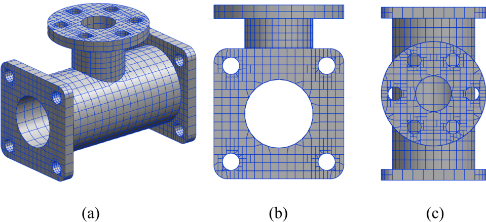
Fig. 34. Results of three-way pipe meshed by BTM:(a) Front view; (b)Side view; (c)Top view.
