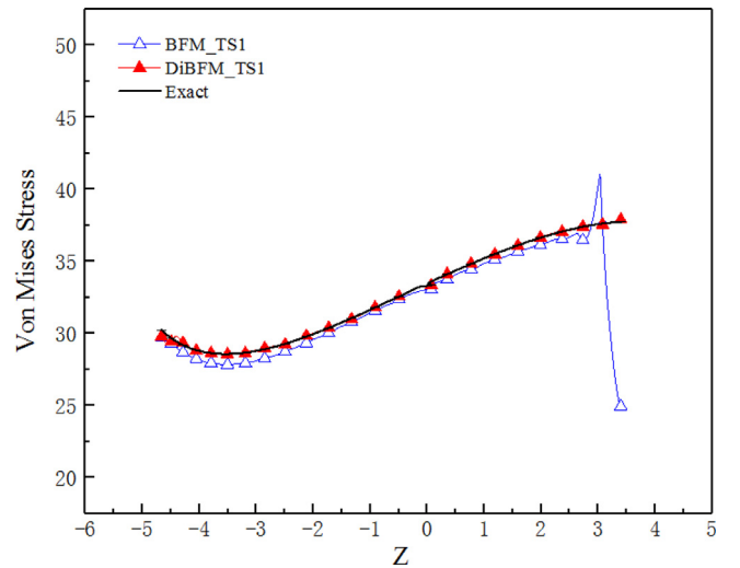
Fig. 20. Von Misses stress along the curve AB.
