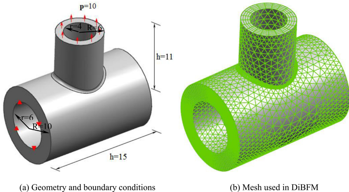
Fig. 22. Three-way pipe.
