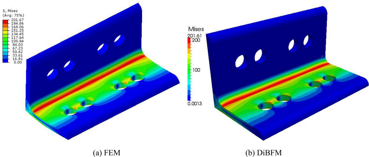
Fig. 28. The Von Mises stress results by the two methods.
