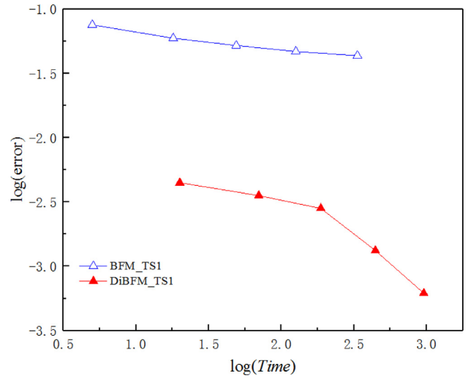
Fig. 21. Comparison of computational efficiency for Von Misses stress.
