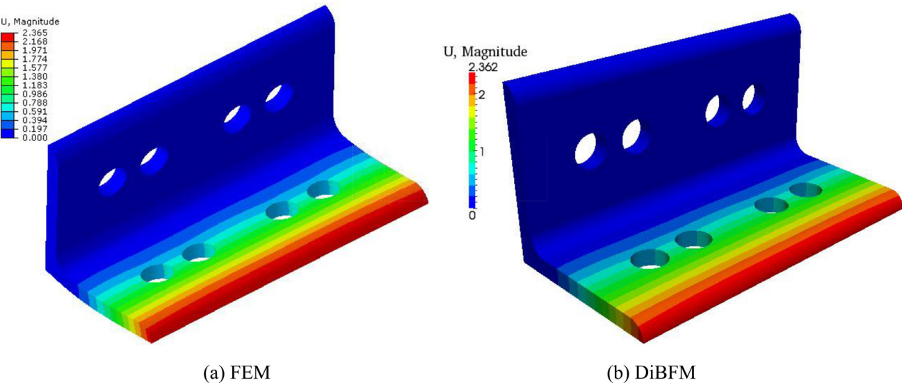
Fig. 27. The displacement results by the two methods.
