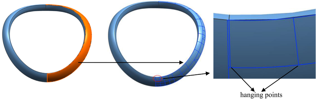
Fig. 4. Face discretized by discontinuous grids.
